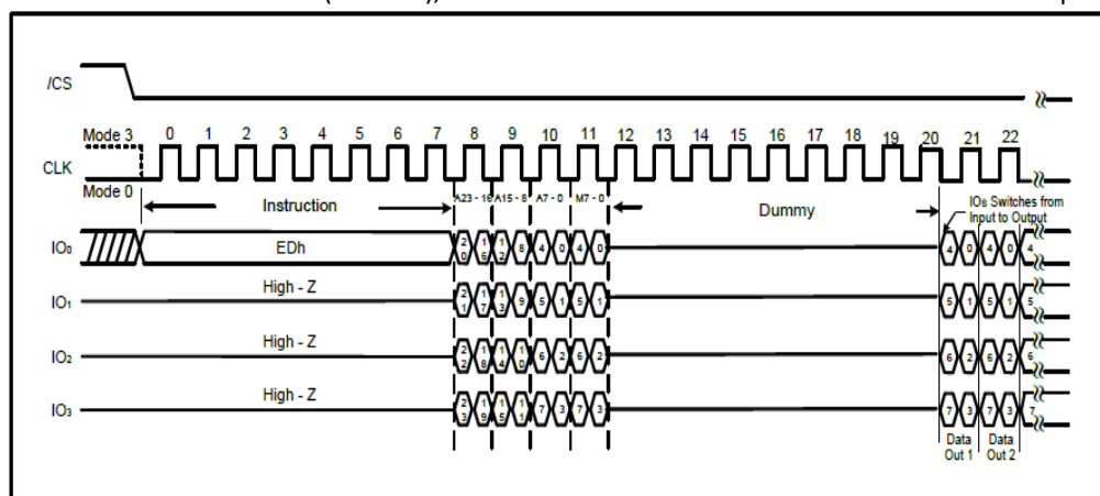
Figure18f. DTR Read Quad I/O Instruction (Previous instruction set M5-4 \neq 10, SPI Mode)
